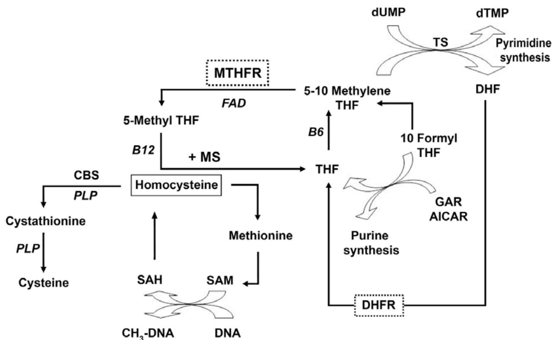
Figure 1. Hcy metabolism and involved vitamin determinants. Hcy is an intermediary in sulfur amino acid metabolism. The methionine cycle and the folate cycle are involved in Hcy formation via the numerous methyl transfer reactions. The metabolism of Hcy is also dependent on several vitamins, including folate, B12 (cobalamin), B6 (pyridoxine). AICAR, aminoimidazolecarboxamide ribotide; CBS, cystathionine beta-synthase; DHF, dihydrofolate; DHFR, dihydrofolate reductase; FAD, flavin adenine dinucleotide; GAR, glycinamide ribotide; MS, methionine synthase; MTHFR, methylene tetrahydrofolate reductase; PLP, pyridoxal phosphate; SAH, S-adenosylhomocysteine; SAM, S-adenosylmethionine; THF, tetrahydrofolate; TS, thymidylate synthase.
